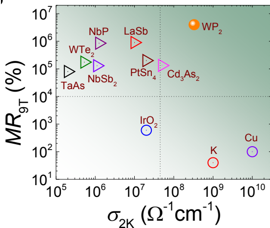
Graph of MR vs. conductivity of some well-known metals and semimetals plane at 2 K and 9 T for comparison. Semimetals are denoted by triangles, metals by hollow circles and WP 2 by a solid circle. Metals with high conductivity have smaller MR and semimetals with smaller conductivities have larger MR. WP 2 exhibits both very large conductivity as well as extremely high MR.
